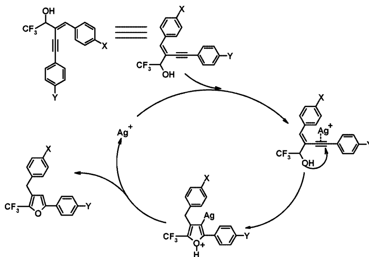
Scheme 3. A tentatively proposed catalytic cycle for the formation of 5 .
