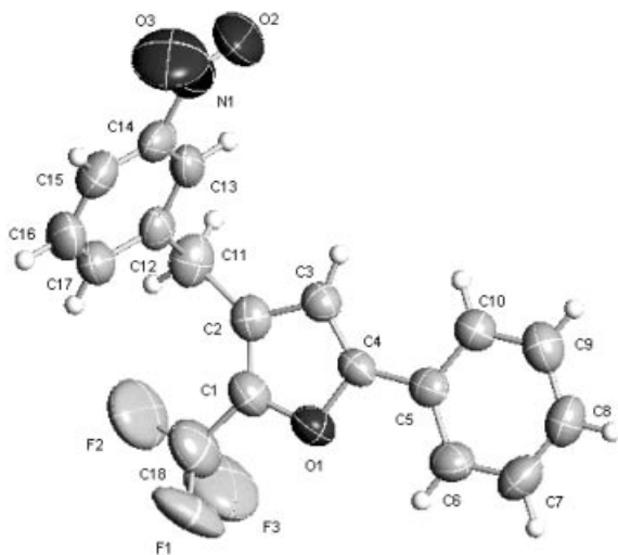
Figure 1. Crystal structure of compound 5h .
