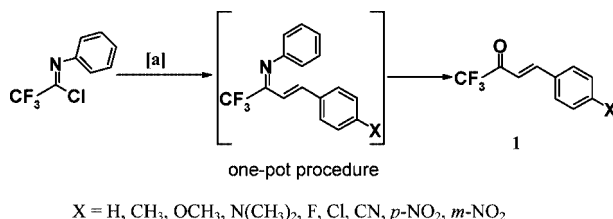
Scheme 1. Reagents and reaction conditions: [a] LDA (2 equiv.), −70 °C; then CH 3 P(O)(OEt) 2 /ArCHO; then 2 N HCl, 4 h.
